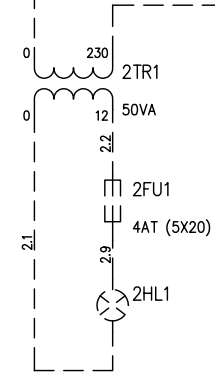
LUCE CAMERA CHAMBER LIGHT
