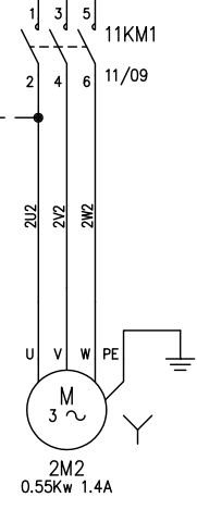
POMPA GIRANTI WASHING ARMS PUMP
