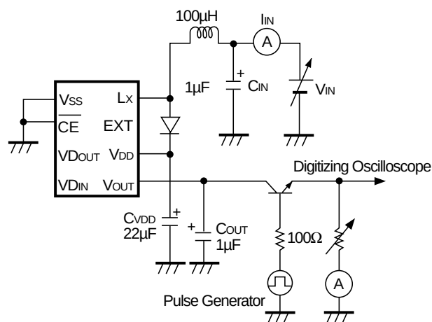
Test Circuit 6
