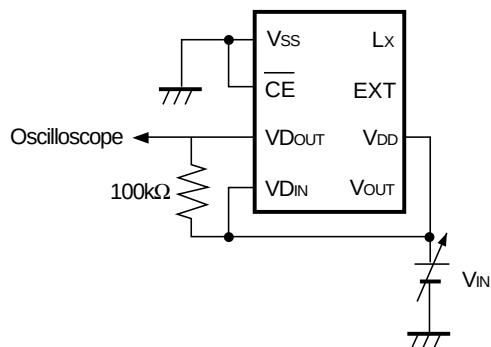
Test Circuit 2
