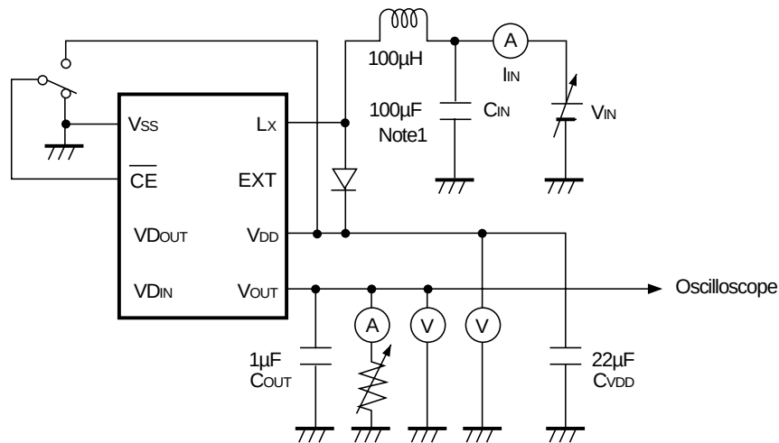
Test Circuit 1
