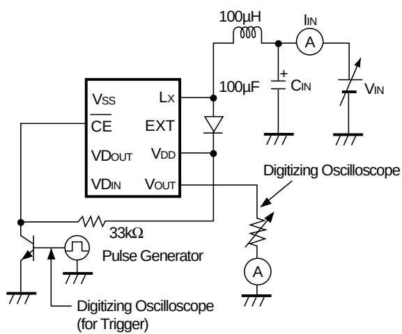
Test Circuit 4
