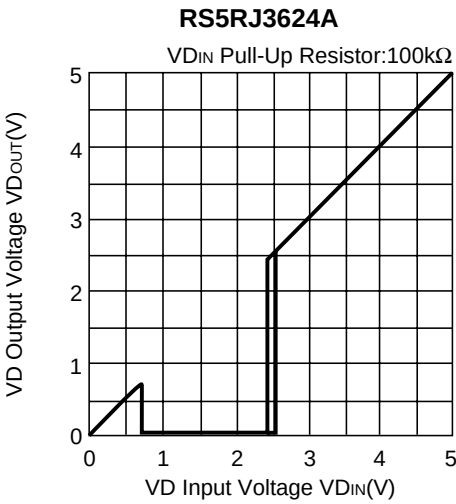
12) VD Output Voltage vs. VD Input Voltage
