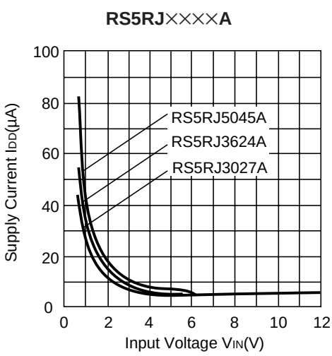
13) Supply Current vs. Input Voltage
