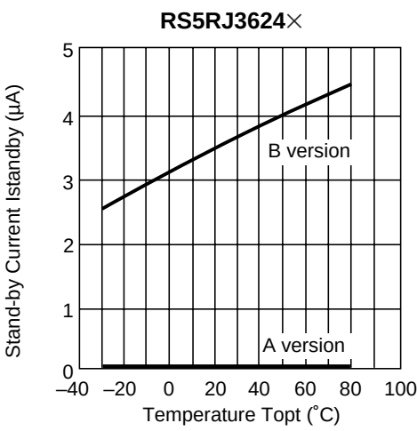
14) Stand-by Current vs. Temperature
