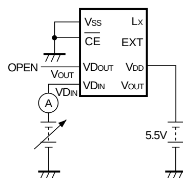
Test Circuit 5
