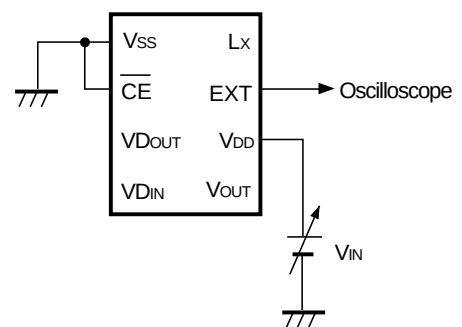
Test Circuit 3
