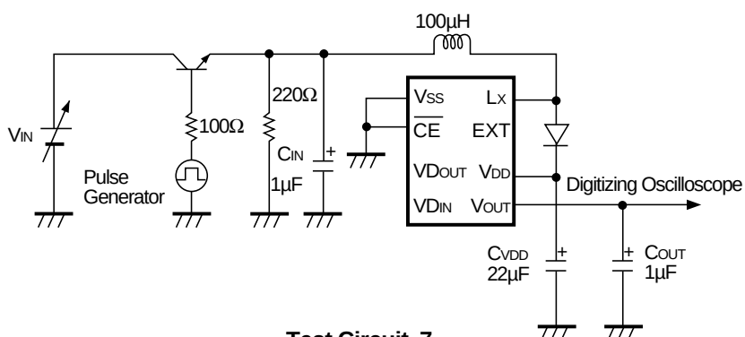
Test Circuit 7
