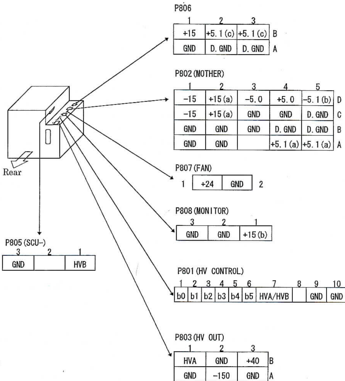
Fig.6-13 Location of connectors
