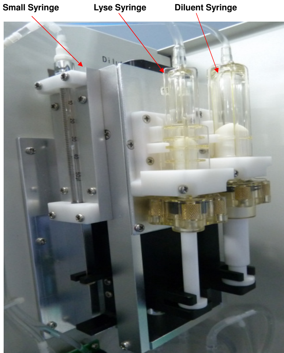
Figure 4-2 Dilutor
