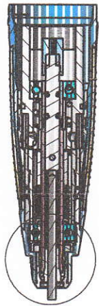
B-B (1:1)
