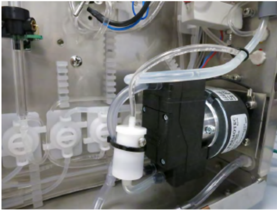
Waste pump
