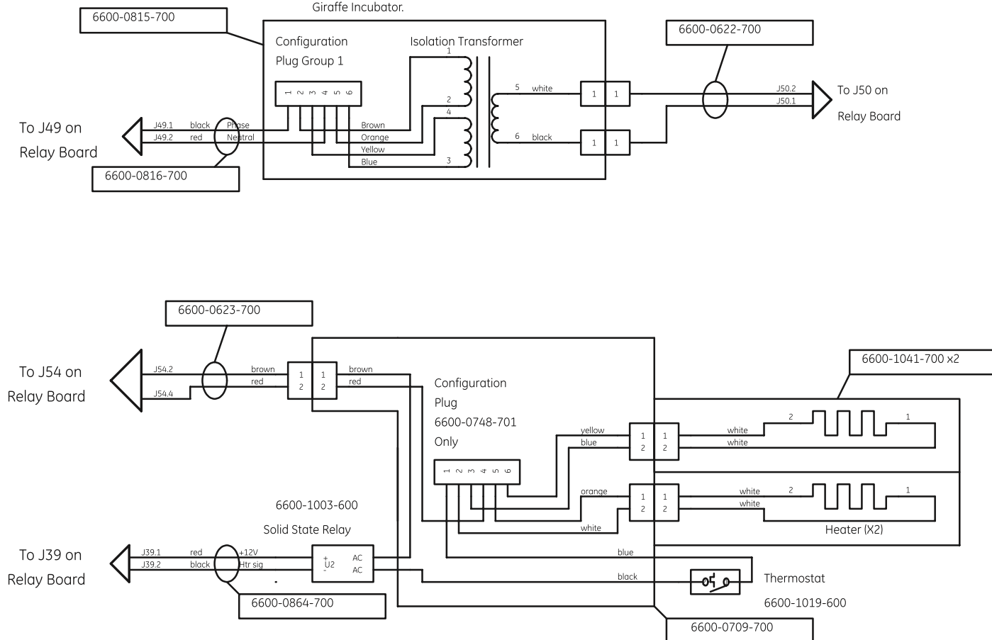
Figure 6-40 Wiring Diagram: Incubator Heater, Relay Board Rev. Level 10 or Higher
