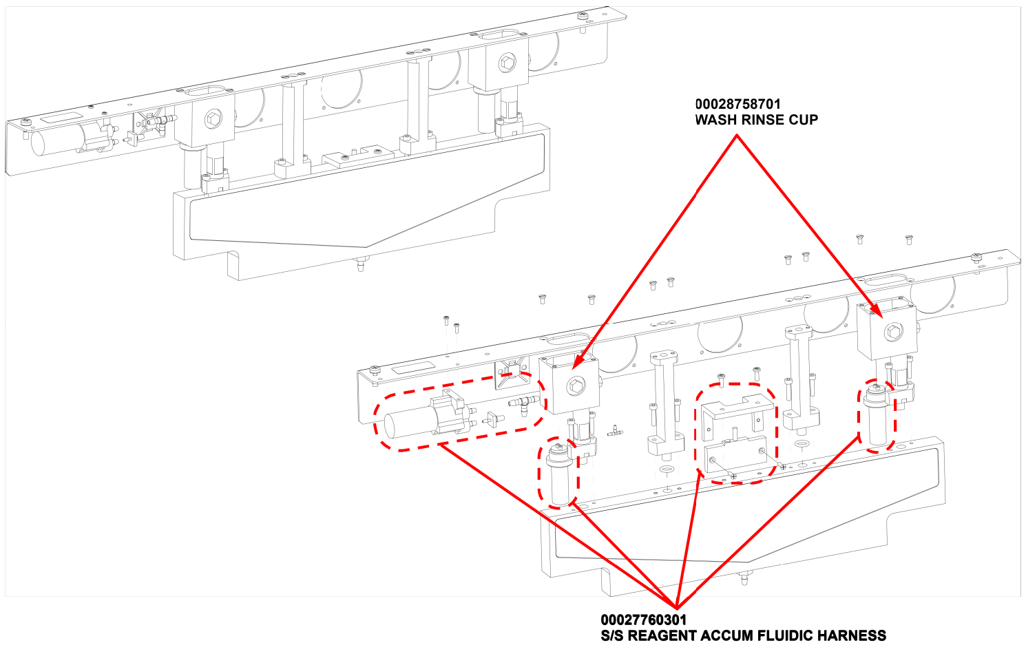
Figure 17-39 28759601 ASSY, CWR STATION, REAGENT
