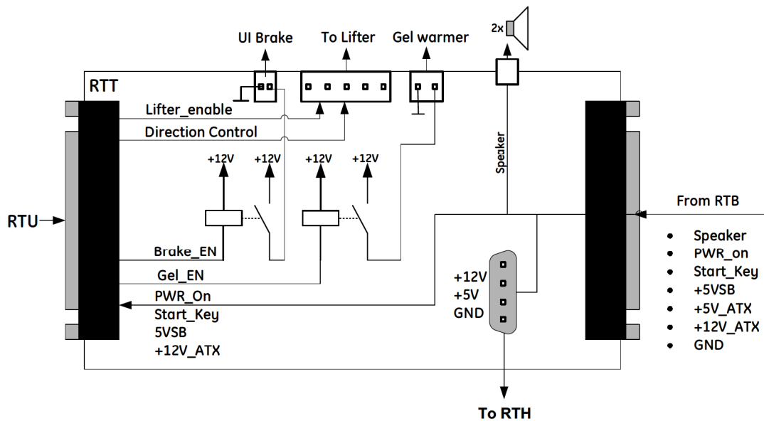
Figure 5-27 RTT - Block diagram
